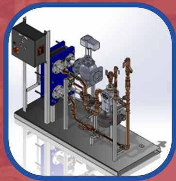
PACKAGED UNIT
